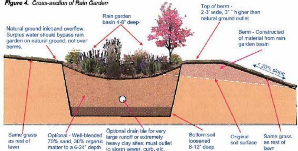
Figure 4. Cross-section of Rain Garden
