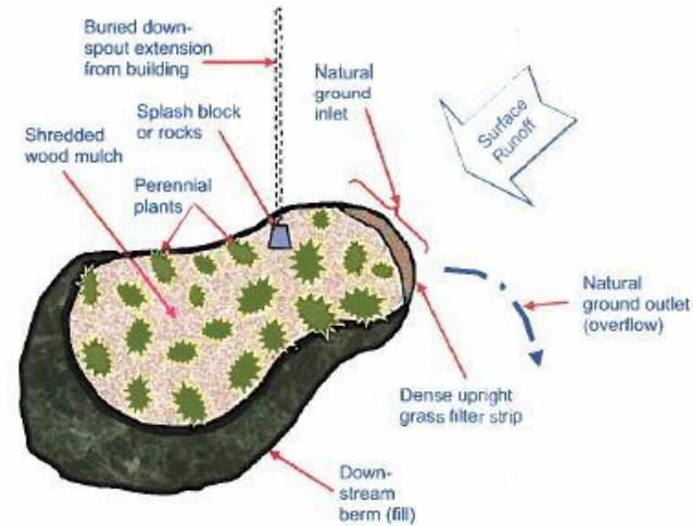
Figure 3. Plan View of Rain Garden
